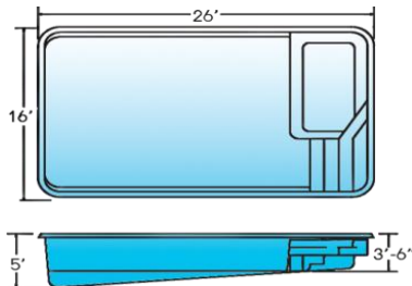
Wilmington - 16'x26'
